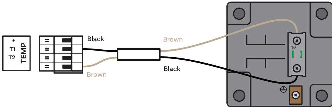
BRB10 button body after disassembly of the top part
