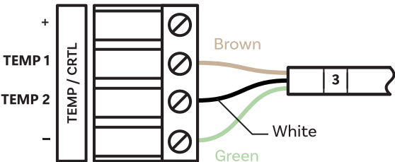
TEMP standard plug-in terminal block
