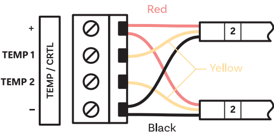
TEMP screw terminal block (directly on digital clock PCB)
