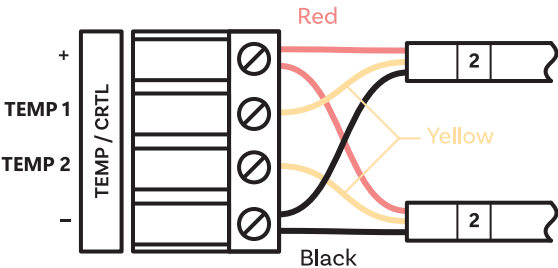
TEMP standard plug-in terminal block
